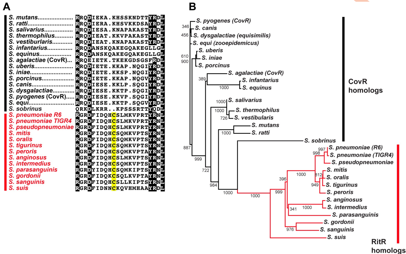
Fig 5. Conservation of RitR in the streptococci. (A) Alignment of linker regions of RitR homologs (in red) and CovR homologs (in black) from the streptococci. Notice the degeneracy in the “HCS” motif in the swine zoonotic pathogen S. suis . Identical residues are colored black and similar residues are colored grey. The conserved cysteine is shaded in yellow. (B) Phylogenetic tree of RitR (in red) and CovR (in black) streptococcal homologs. Evolutionary distance is depicted by the length of the horizontal lines. Posterior probabilities are displayed at the branch points.
