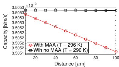
Fig. 18. Channel capacity versus distance between two antennas
