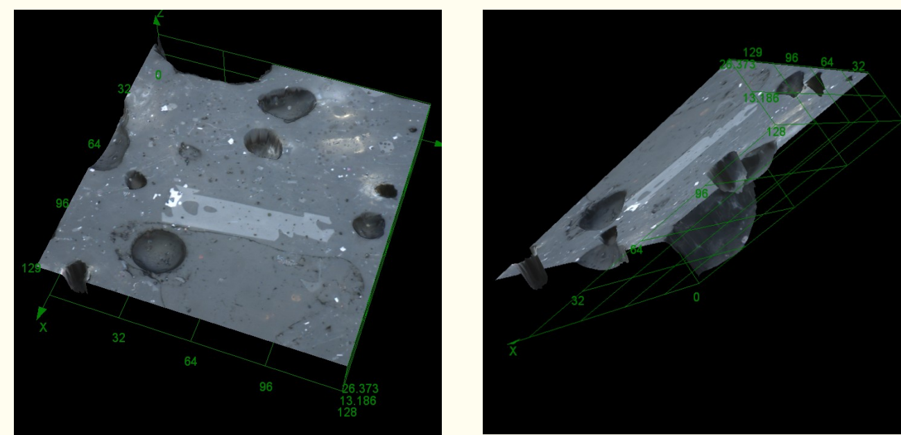
Example of views of thick section from Eyjafjallajökull sample 128x128x26µm (x100 objective).
